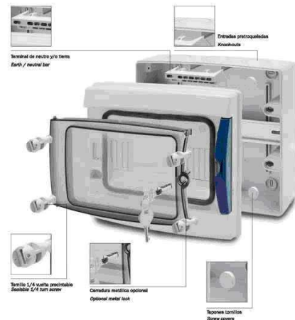
Model 3926-T
